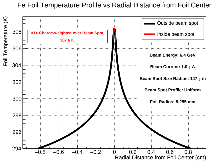
Figure 6: Fe foil temperature profile from integrating Eq. 23 with beam spot size, and energy given.
