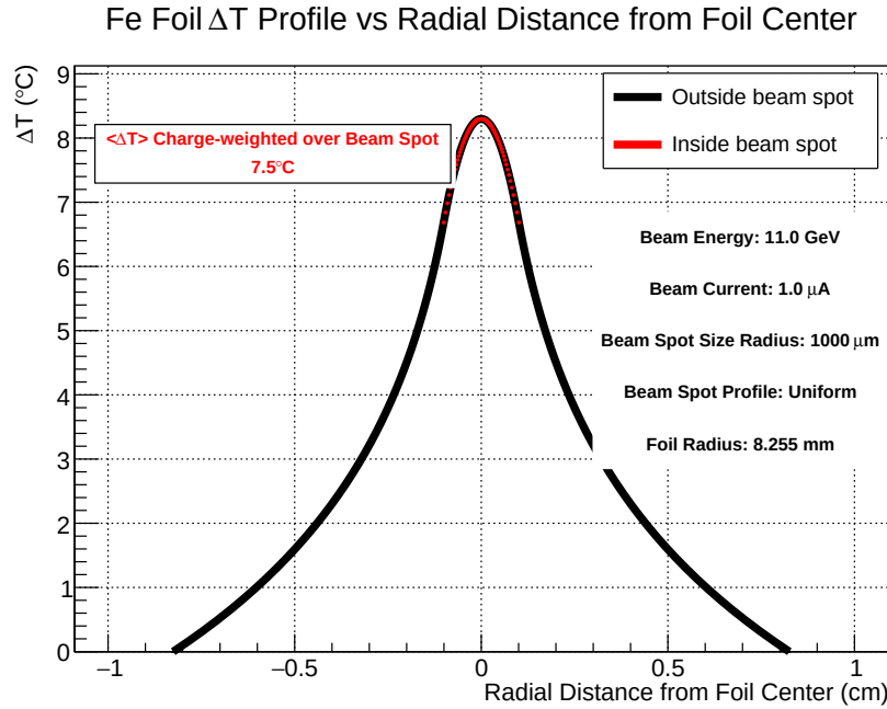
Figure 5: Fe foil \Delta T profile from using Eq. 23 with beam spot size, and energy given.
