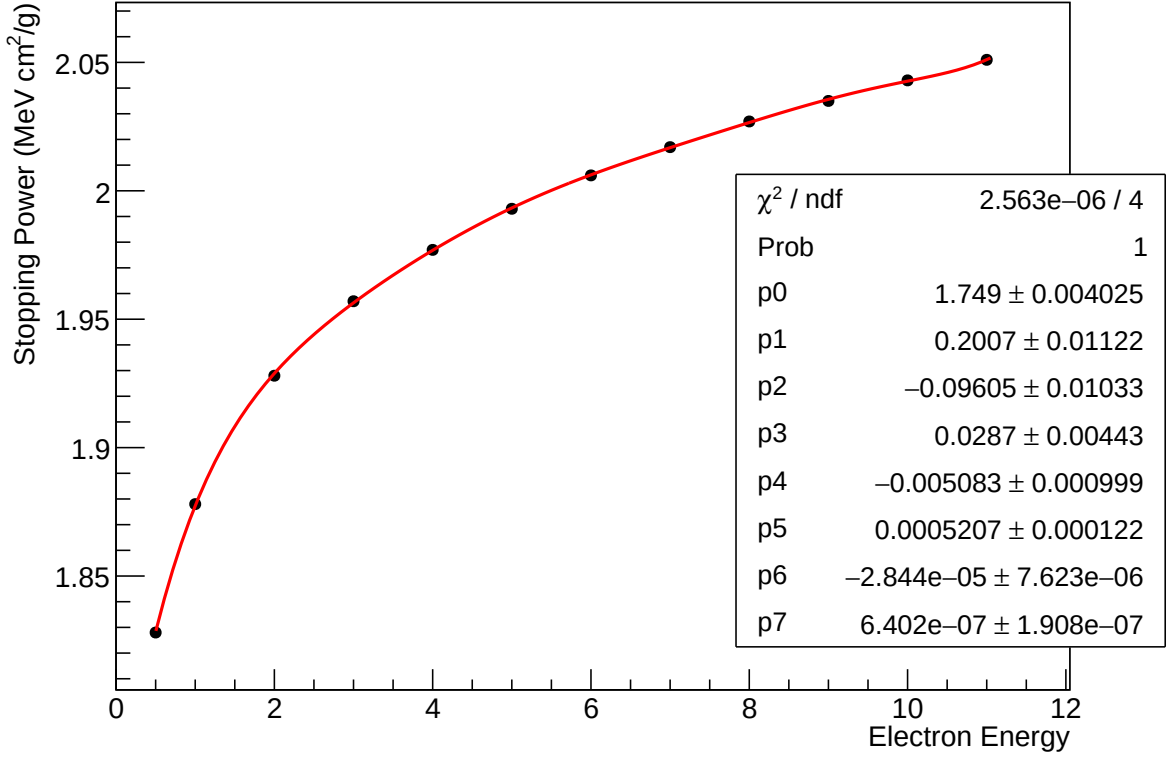
Figure 2: Stopping power for electrons as a function of energy in Fe. Data are from ESTAR and are fit to a 7-degree polynomial.
